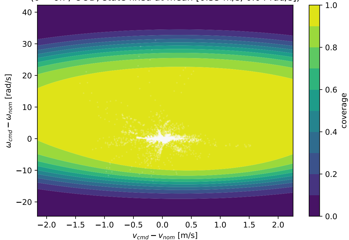
Residual coverage vs command offset (0 = off / OOD; state fixed at mean [0.35 m/s, 0.04 rad/s])
